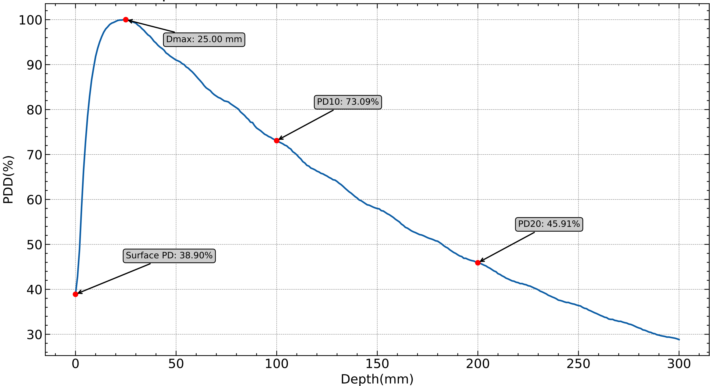
PDD profile of 10MV SSD=100, Water Phantom, F.S= 10x10cm 2
